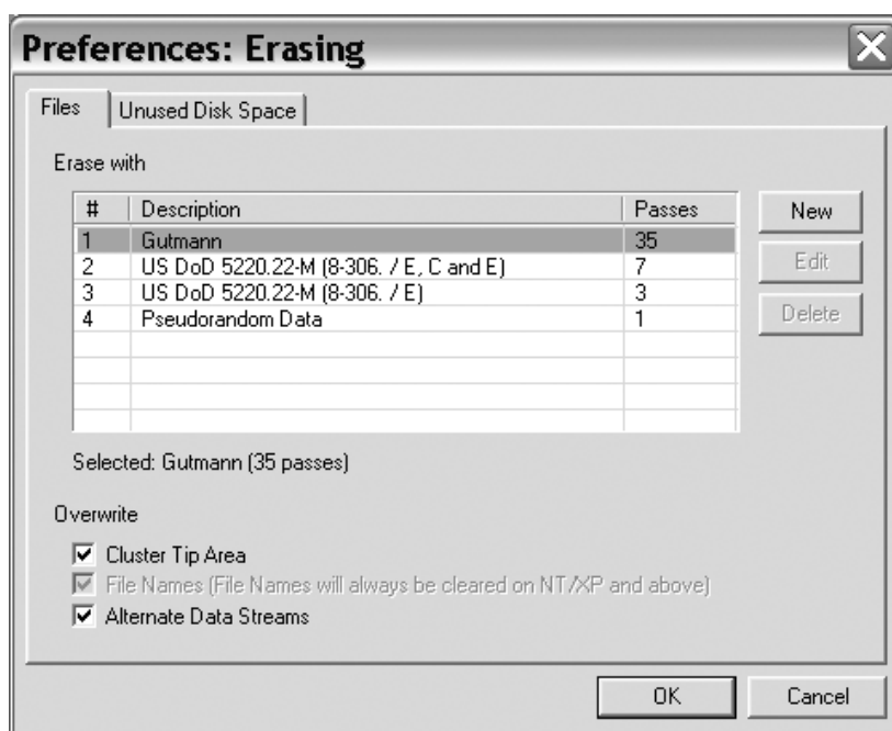
Fig. 2.3: Available settings in a common Windows file erase utility, showing options for various Department of Defense standards-compliant overwrites, as well as the 35 Gutmann patterns.
